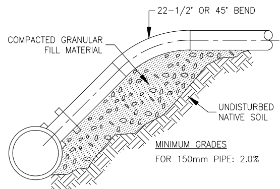
SEWER SECTION
