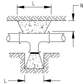
TEE WITH PLUG
