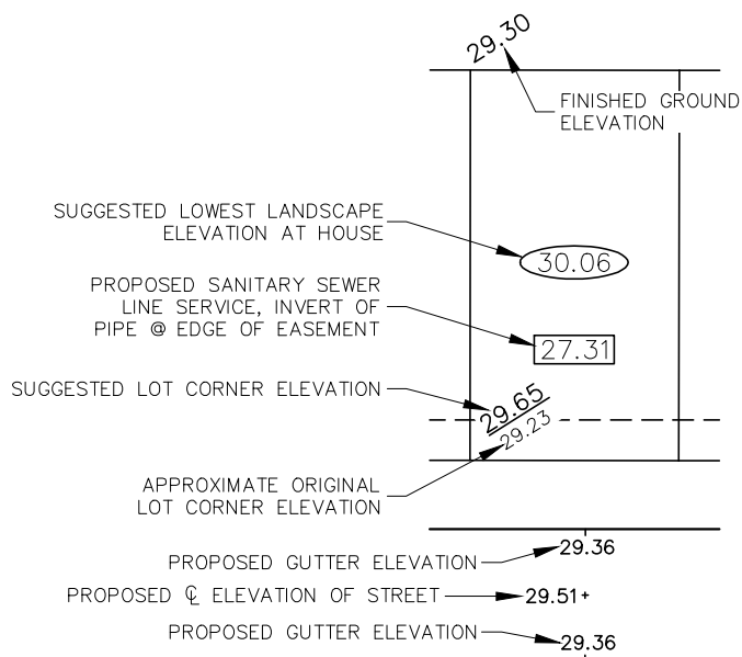
TYPICAL LOT GRADING SECTION
