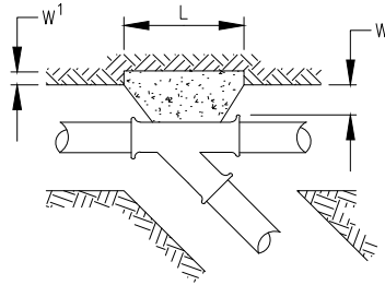
WYE
