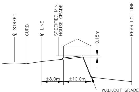
WALKOUT OR BACKSPLIT HOUSE TYPE
