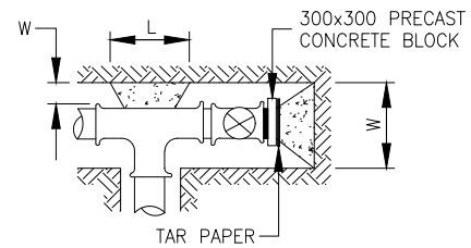
TEE WITH VALVE
